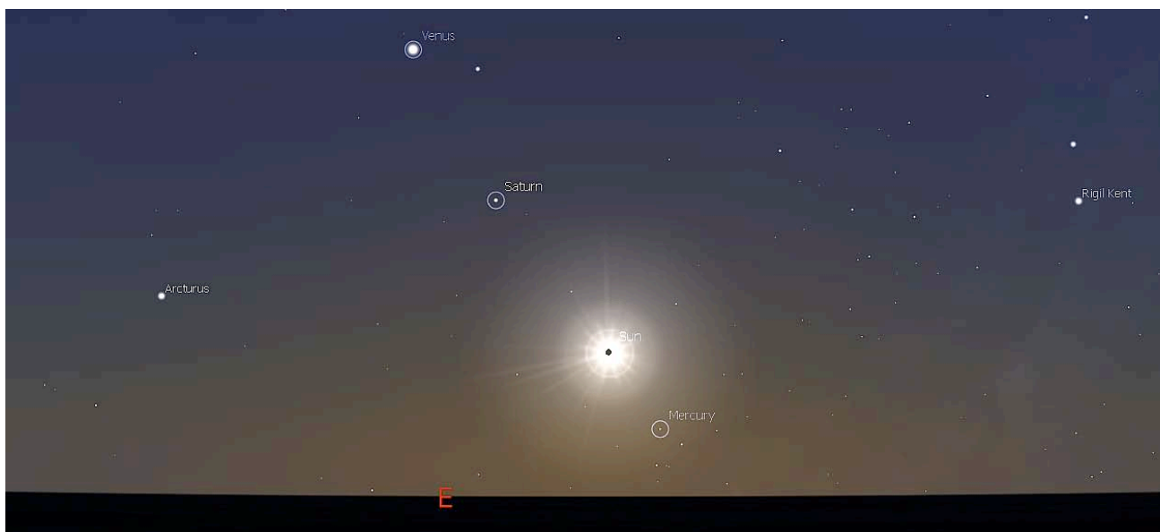
Figure 3 – The sky during totality as seen from Cairns, Queensland at 6:39 am AEST on 14 November 2012. Image: Nick Lomb using Stellarium ( http://www.stellarium.org/ ) software.
